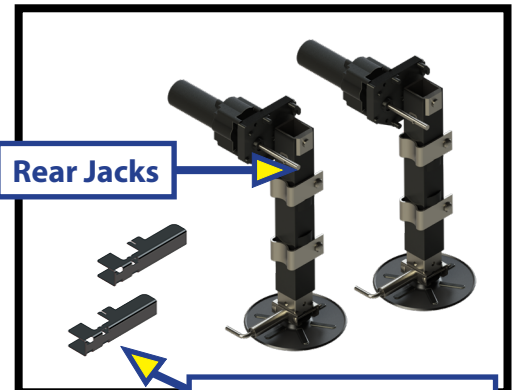
Mounting Brackets
