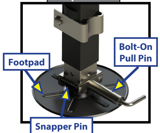
Footpad Detail
