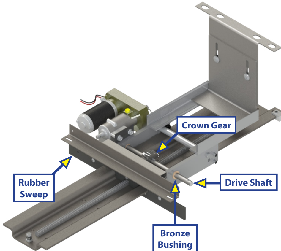
Underside View
