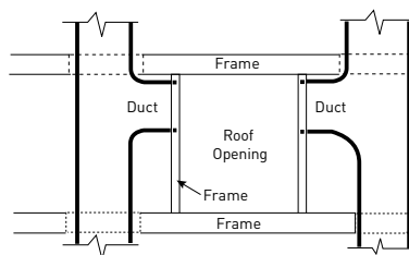
SIDE VIEW (TOWARD BACK OF RV)
