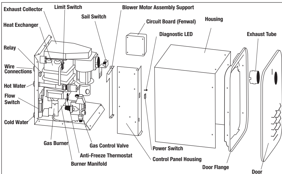
Figure 9 - EXPLODED VIEW OF MODEL GSWH-1 AND MAJOR COMPONENTS IDENTIFICATION
