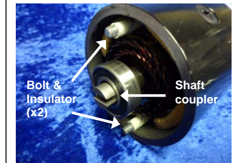
Figure 24 Motor showing bolts, insulators, and shaft coupler
